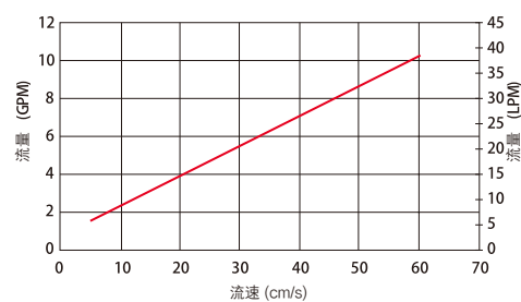
1-1/2" NPT 端口
